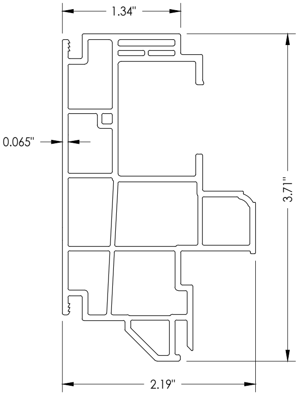
1 FRAME
