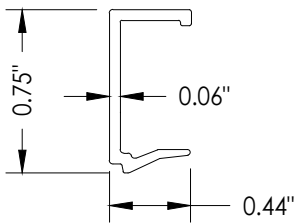
2 GLAZING BEAD
